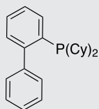
CyJohn Phos SC-5007 247940-06-3
