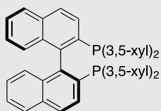
(S)-XyIBINAP
