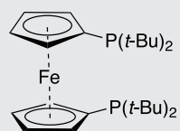
DtBPF
