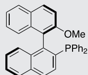
(R)-MOP
