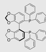
(S)-(-)-SEGPPOS
