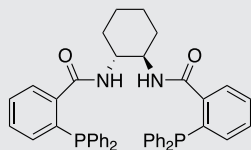
(R,R)-DACH-Phenyl Trost Ligand
