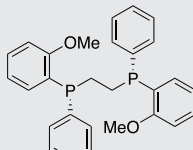
(R,R)-DIPAMP
