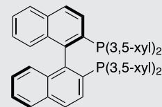
(R)-XyIBINAP
