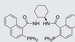
(R,R)-DACH-Naphthyl Trost Ligand
