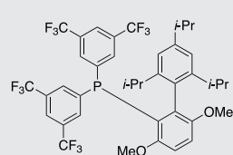
JackiePhos SC-5016 1160861-60-8
