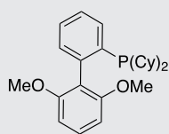
SPhos SC-5001 657408-07-6
