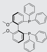
(S)-MeO-BIPHEP
