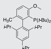
RockPhos SC-5020 1262046-34-3
