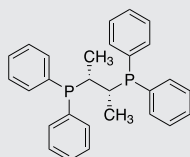
(R,R)-CHIRAPHOS
