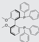
(R)-MeO-BIPHEP
