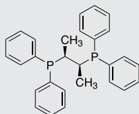
(S,S)-Chiraphos
