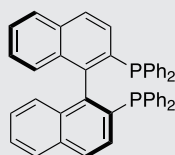
(S)-BINAP
