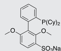
SPhos-SO 3 Na SC-5015 870245-75-3/ 1049726-96-6
