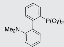
DavePhos SC-5004 213697-53-1
