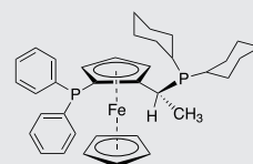
(R)-(S)-JOSIPHOS
