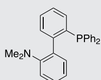
PhDavePhos SC-5012 240417-00-9
