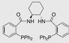
(S,S)-DACH-Phenyl Trost Ligand
