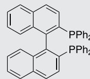
Rac-BINAP
