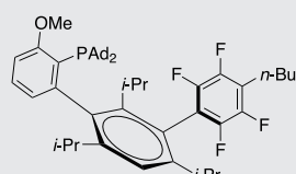
AIPhos SC-5023 1805783-60-1
