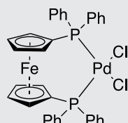
(DPPF)PdCl 2
