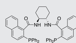
(S,S)-DACH-Naphthyl Trost Ligand
