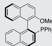
(S)-MOP
