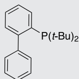
JohnPhos SC-5006 224311-51-7
