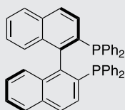
(R)-BINAP
