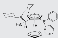
(S)-(R)-JOSIPHOS
